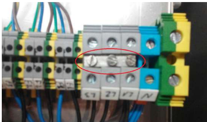
Figure 3.1: Single-phase connection
