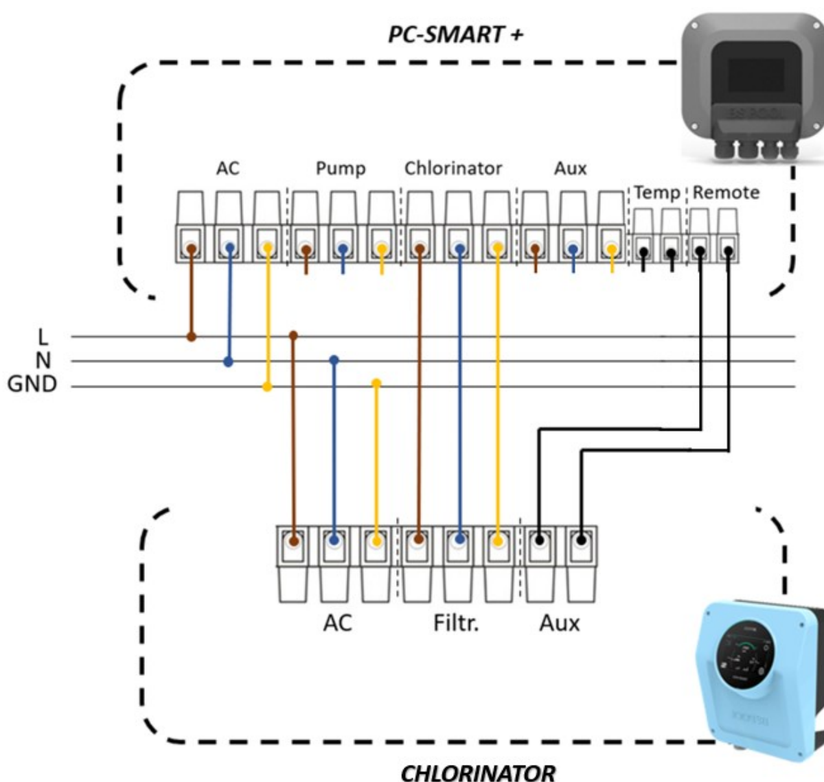
Fig. 4: Example of remote connections.
